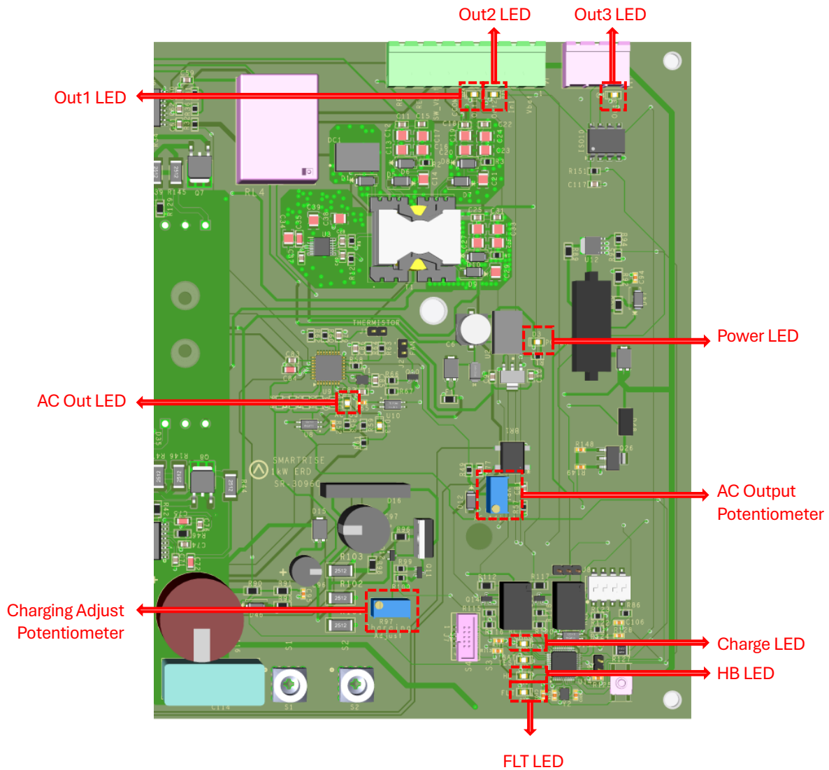
Figure 7: ERD LEDs
