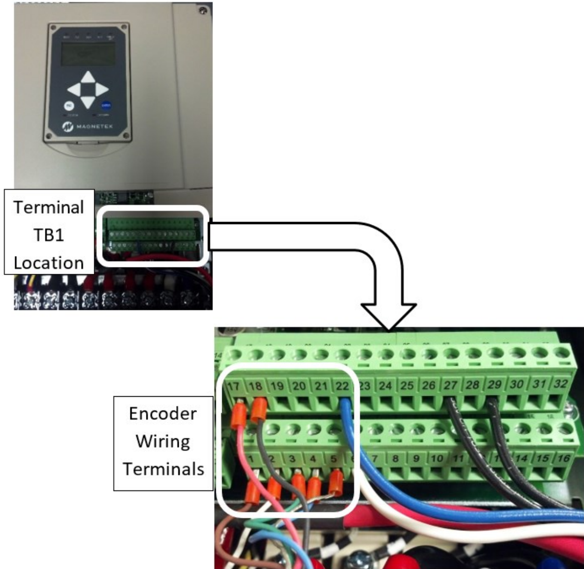
Figure 7: Encoder Terminal Location
